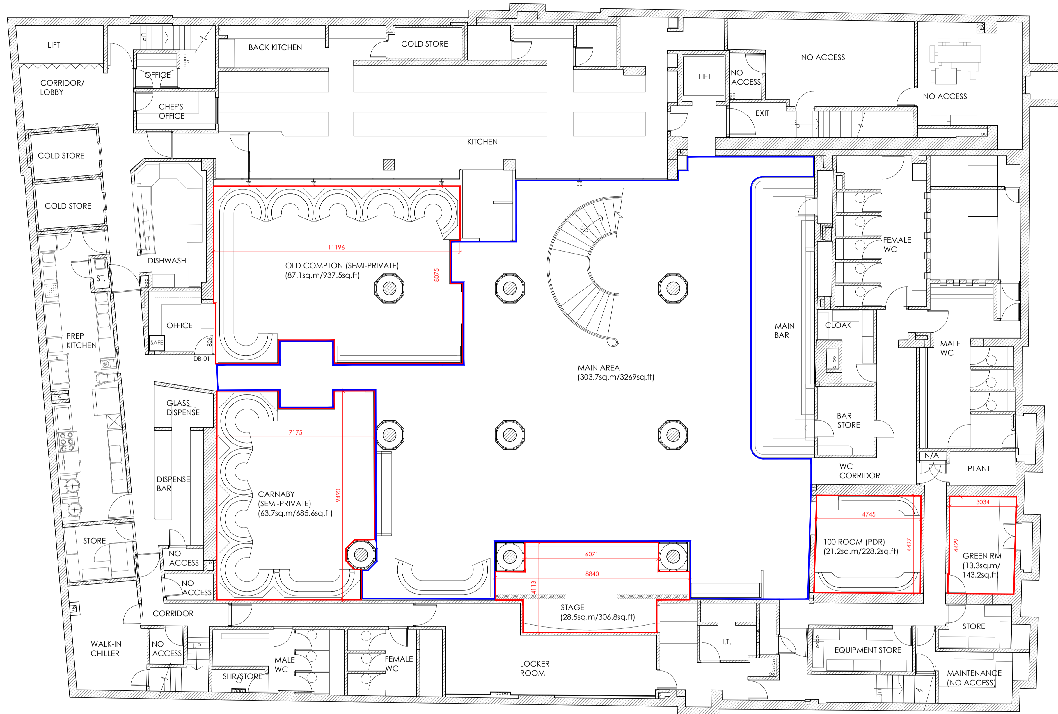
BASEMENT AREAS PLAN SCALE 1:100 @ A1
